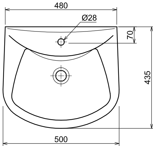
PLAN / TOP ELEVATION
