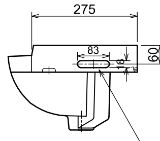
VIEW A
