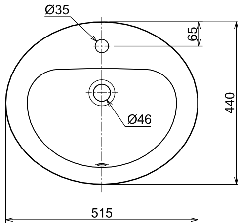
PLAN / TOP ELEVATION
