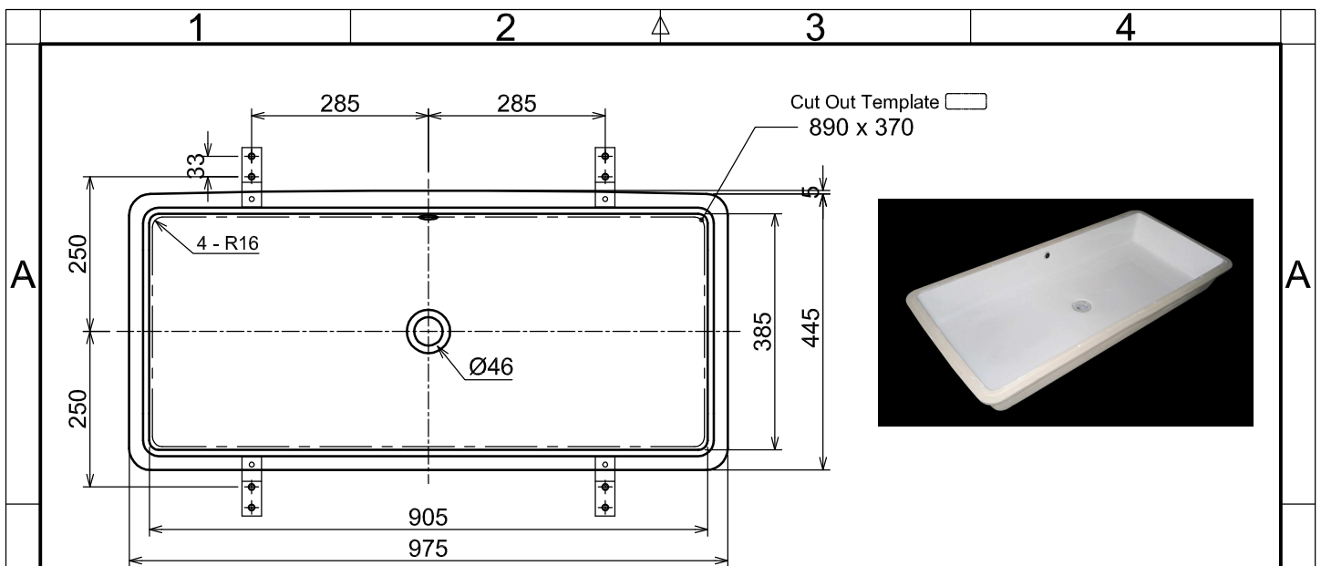
PLAN / TOP ELEVATION
