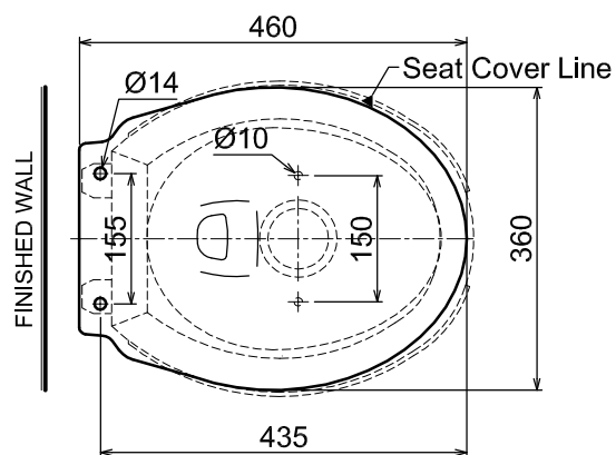
PLAN / TOP ELEVATION
